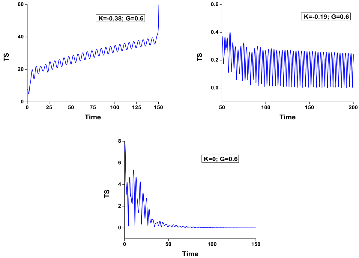
Figure 3.: Time histories of TS displaying synchronized states: Upper and middle panels show instability of the process while lower panel shows full synchronization
